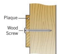
Through The Face Mount
